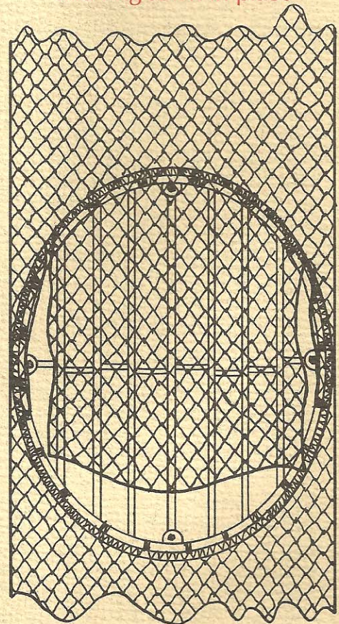
Bottom View "Georgia Jumper" with grid and ring sewn in place
